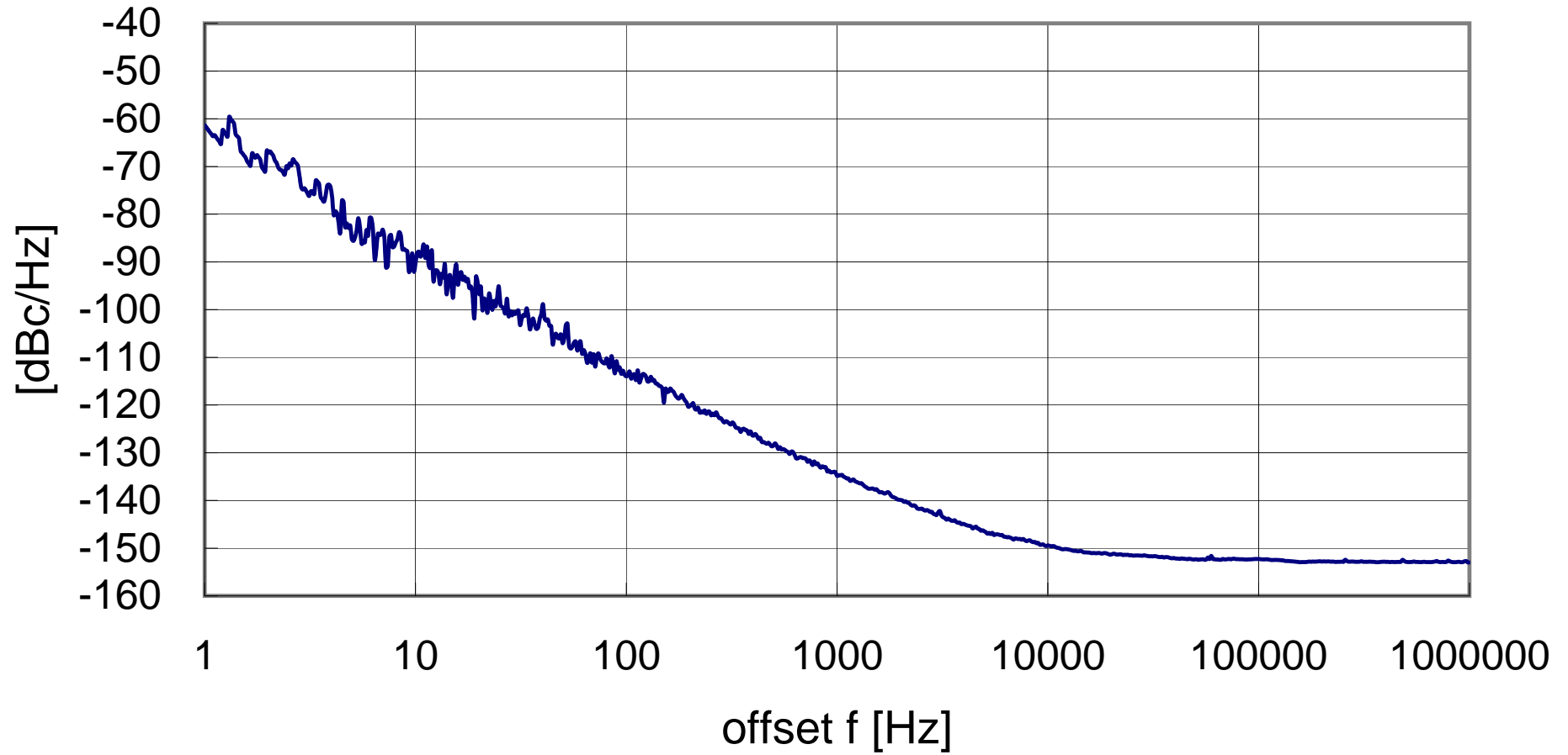
NT2016SA Phase Noise (26MHz)
