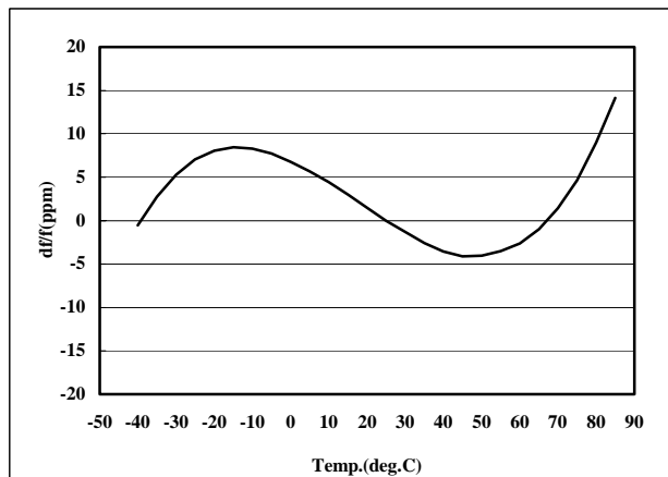
Figure.4 Typical frequency-temperature characteristics
