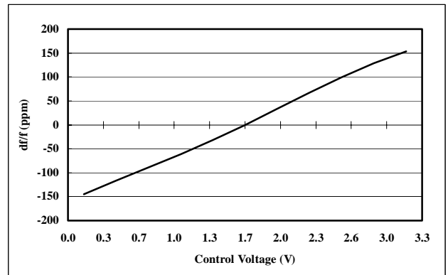
Figure.5 Typical frequency-control voltage characteristics
