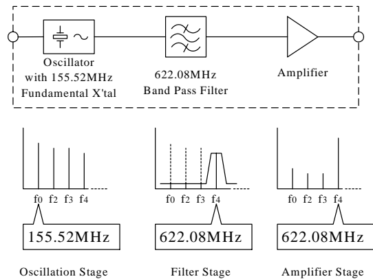
Figure 2 Construction and function block diagram of this new oscillator
