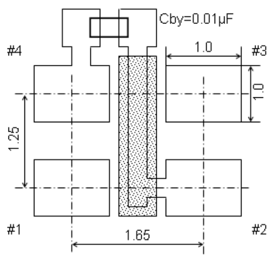
Land pattern (Recommended)
